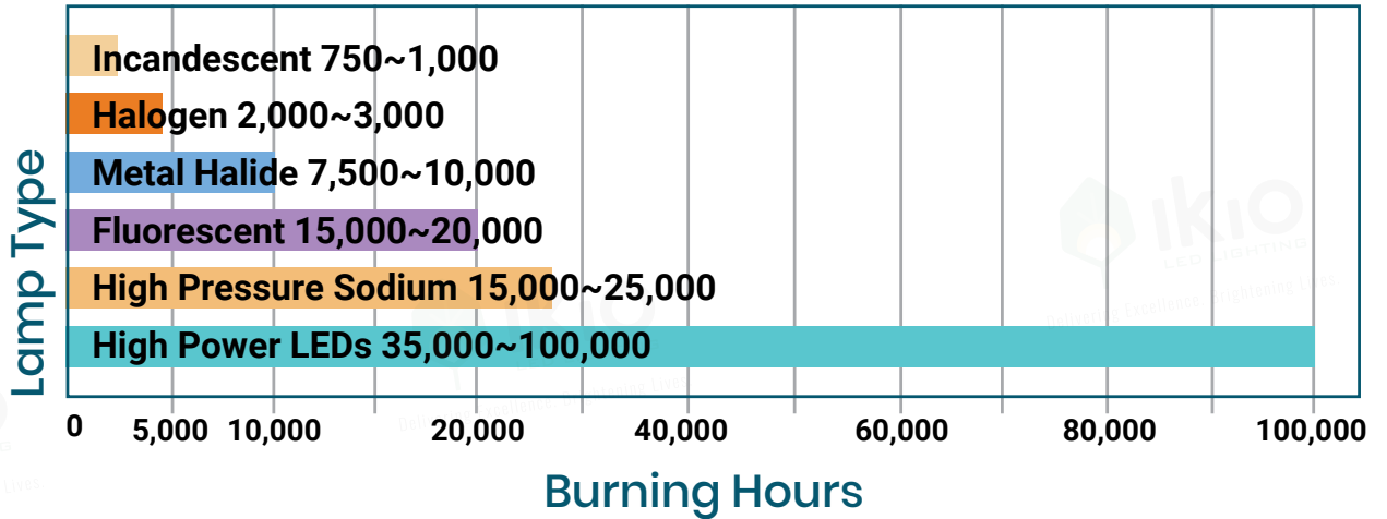
Figure 26. Typical lamp lifespan
