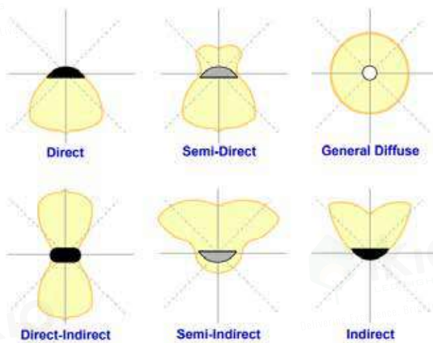
Figure 145. The various light distribution strategies
